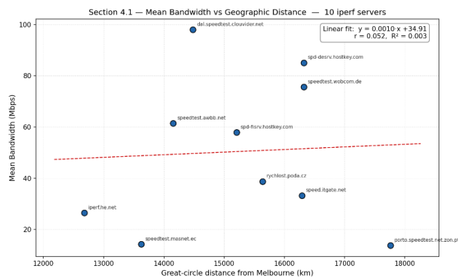
<Fig 4.1.3 Scatter chart and fitted linear for mean Bandwidth VS Distance>
